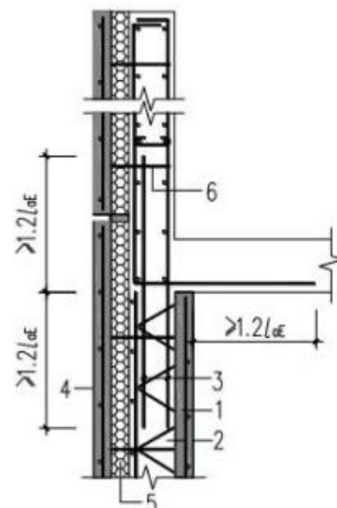
(b) 叠合剪力墙与现浇女儿墙 (不等厚)
