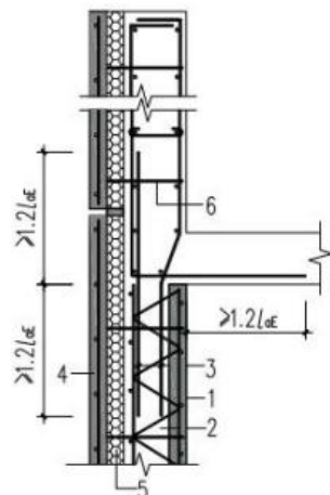
(a) 叠合剪力墙与现浇女儿墙 (等厚)
