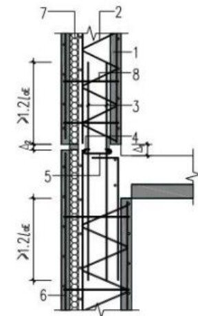
(c) 叠合剪力墙 (不等厚, a/b > 1/6 )
