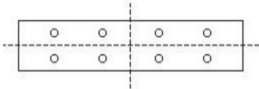
图 C.3 条缝形风口测点布置
