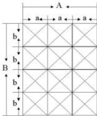
图 C.2 矩形风口测点布置
