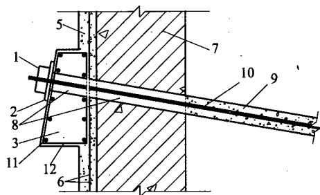
(a) 预应力锚杆、围檩与面层
